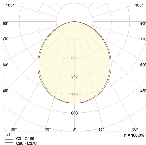
Polar light distribution diagram
