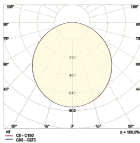
Polar light distribution diagram
